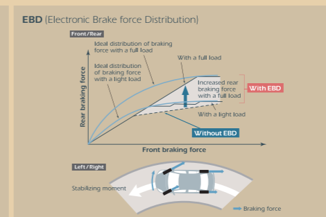
Anti-lock Brake System (ABS) with Electronic Brake-force Distribution (EBD)
